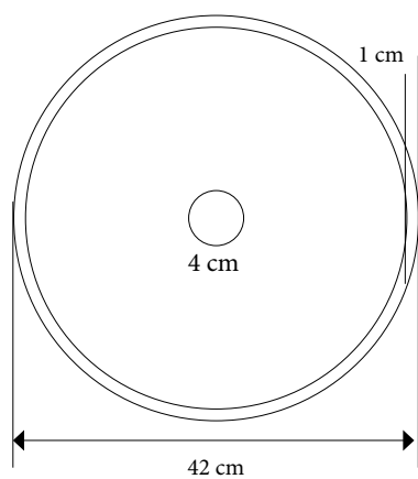
CP950FEEL Lavandino Index Feel
