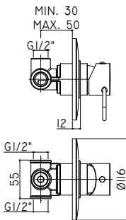
JK 010-011CR Miscelatore incasso doccia / Piastra Ø116 e 110 mm Concealed shower mixer / Wall plate Ø116 and 110 mm
