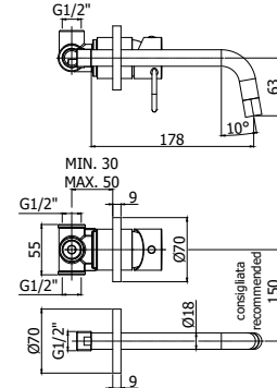
JK 006-007CR70 Miscelatore incasso con bocca erogazione a muro 175 mm / 245 mm Concealed two-hole basin mixer with wall spout 175 mm / 245 mm
